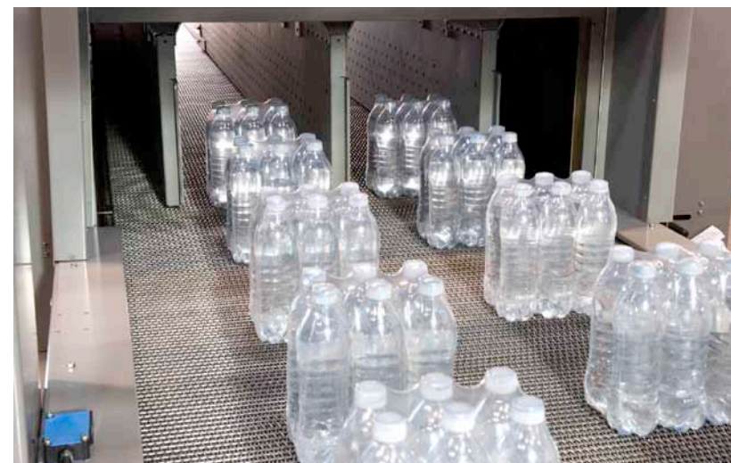
Completed packs leaving the shrinking tunnel.
